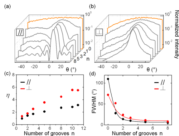
Figure 2. Normalized diffraction patterns in logarithmic scale depending on the groove number n , under parallel (a) and perpendicular polarizations (b). Antenna integrated enhancement factor \eta (c) and main lobe fwhm (d) as a function of groove number n for parallel (black dots) and perpendicular polarization (red dots). In (d) experimental data are compared to theoretical predictions (solid lines).
